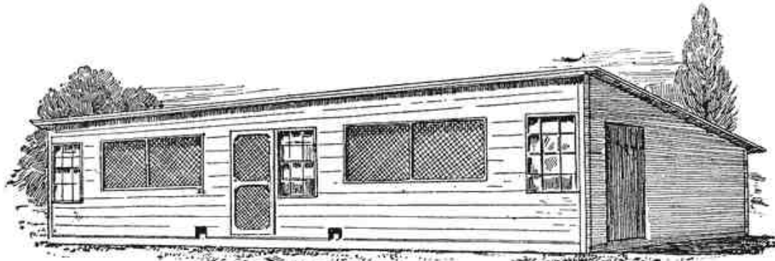
NEW JERSEY MULTIPLE UNIT HOUSE Two units combined to house two hundred fowls
